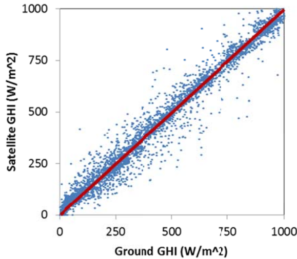
Fig. 1: Irradiance data for Hanford, CA, 2010.
