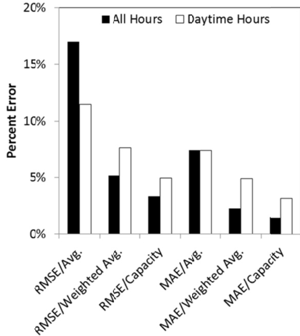
Fig. 2: Comparison of error results for six methods using “All Hours” and “Daytime Hours” for Hanford, CA, 2010
