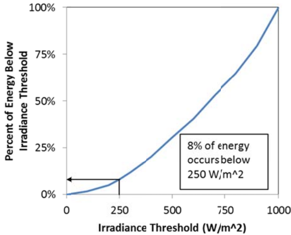
Fig. 3: Energy distribution of irradiance data for Hanford, CA, 2010.
