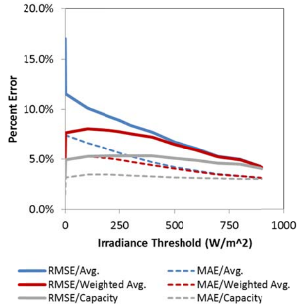
Fig. 4: Comparison of error results for Hanford, CA, 2010.
